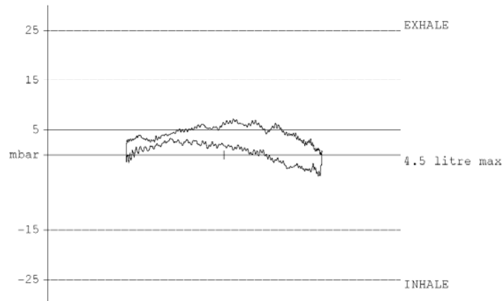
PRESSURE - VOLUME DIAGRAM AT DEPTH OF : 49.8 msw (163,4 fsw)
