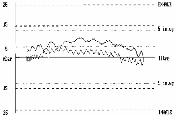
PRESSURE - VOLUME DIAGRAM AT DEPTH OF : 51.0 msw (167 fsw)
